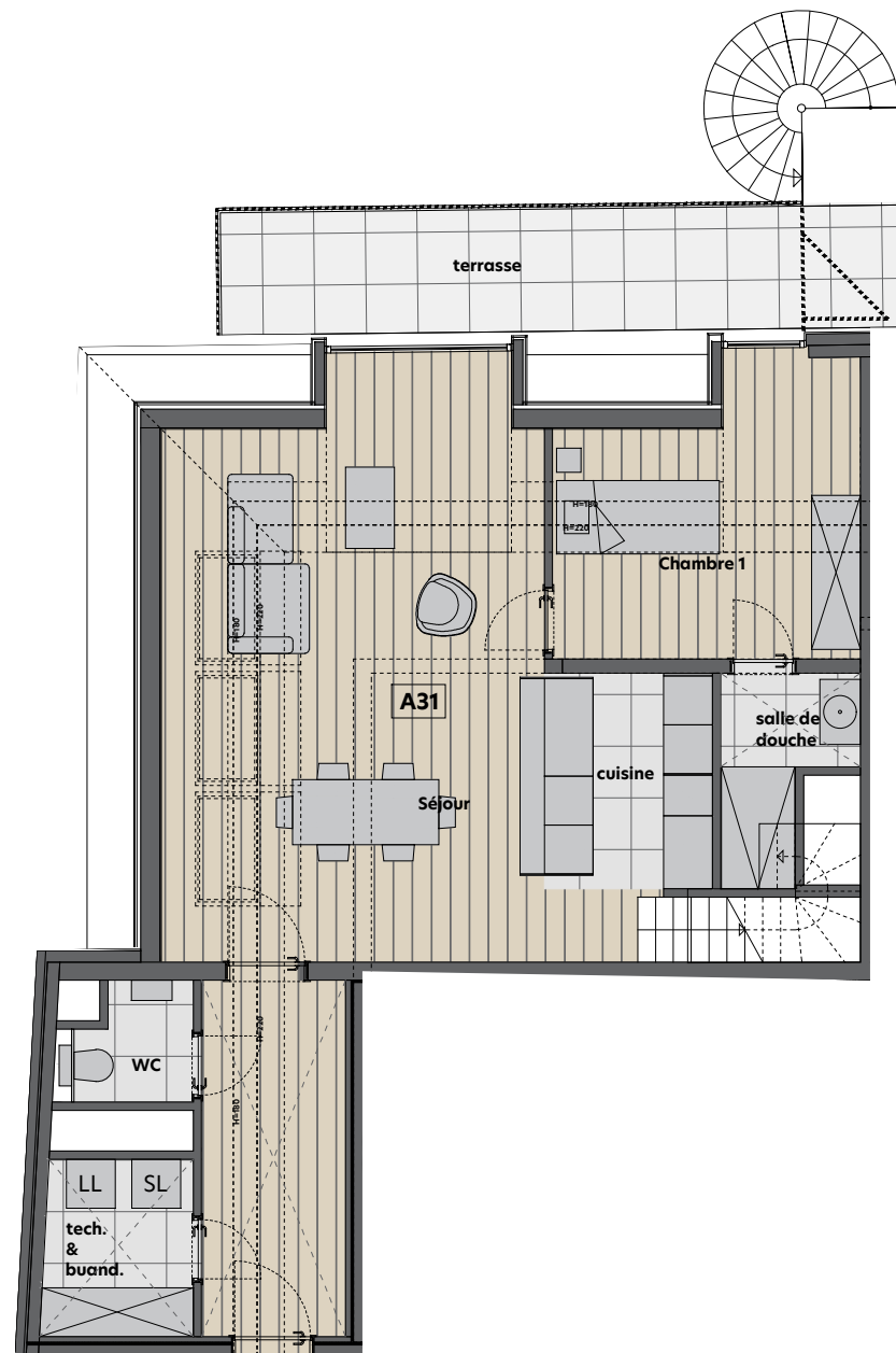
Plan R+3 1/100
