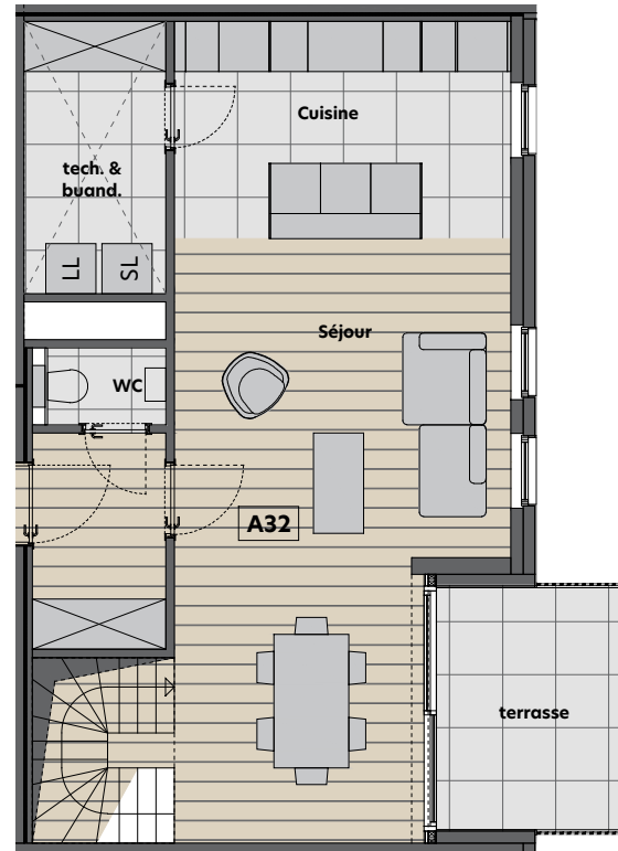
Plan R+3 1/100
