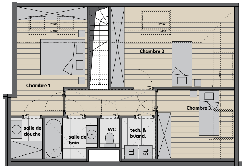
Plan R+3 1/100
